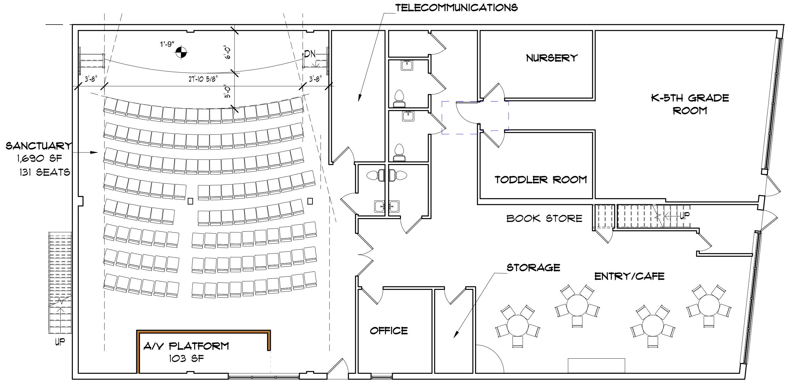
1 A-1 FLOOR PLAN NORTH SCALE: 1/8" = 1'-0" AREA: 4,841 S.F.
